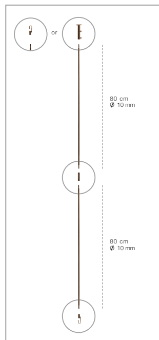
Suspension Kit
