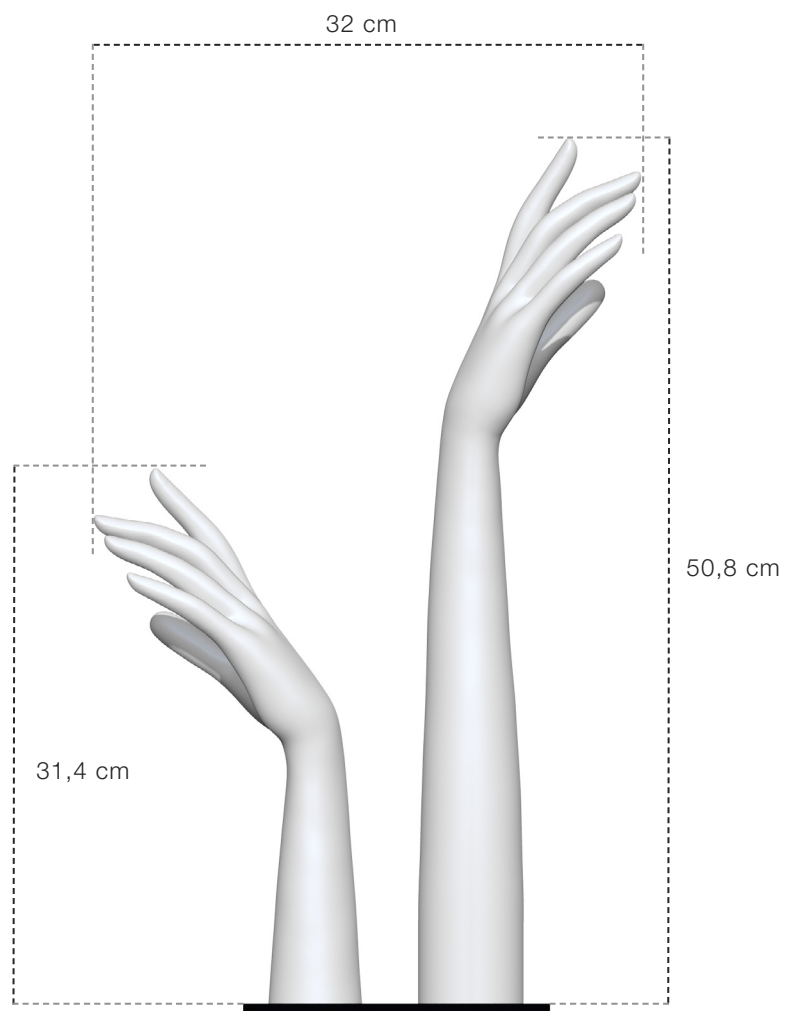
Arm A / Arm B product in 3D printing
